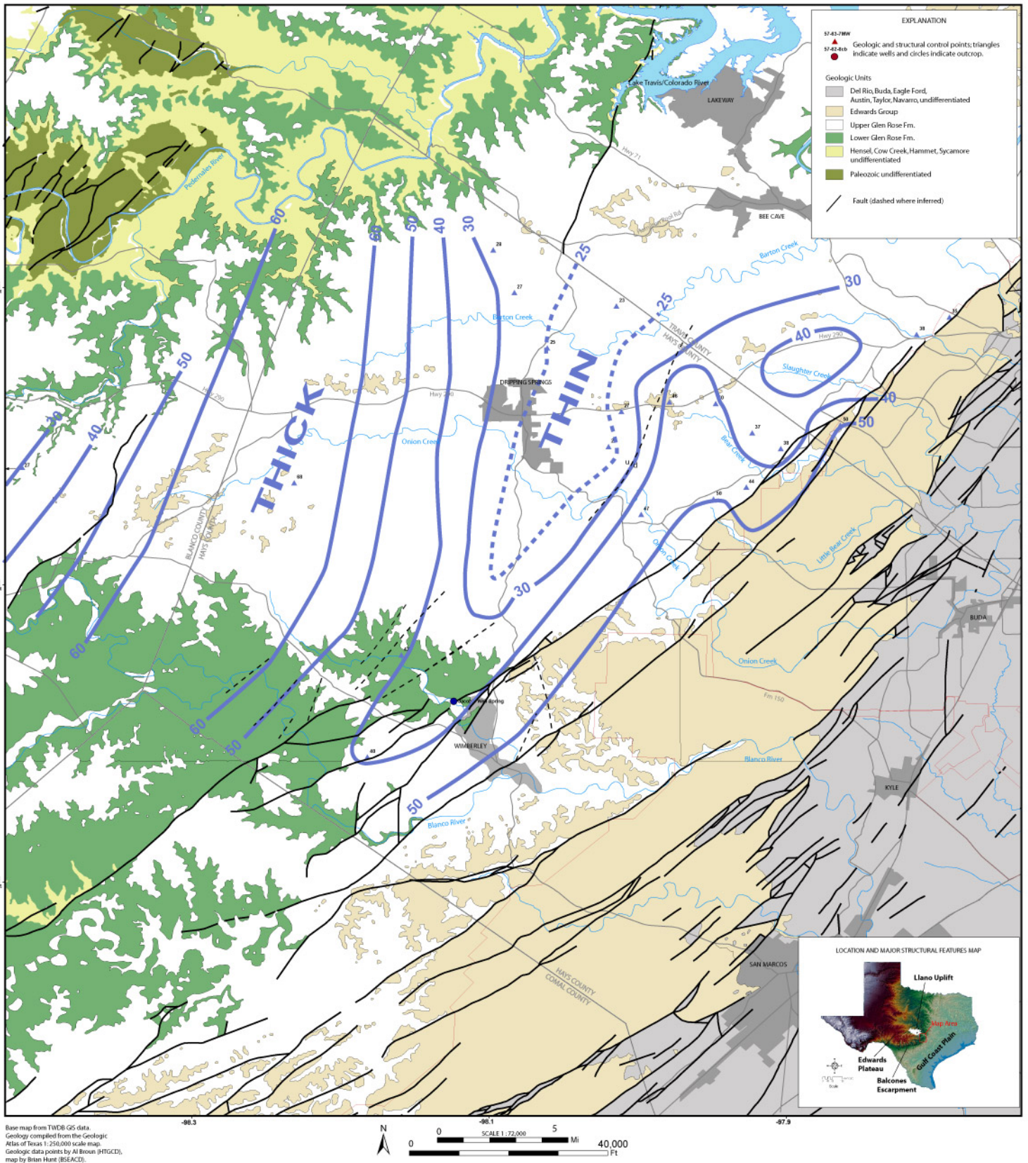
Figure 20. ISOPACH MAP OF THE HAMMETT SHALE March 2007
