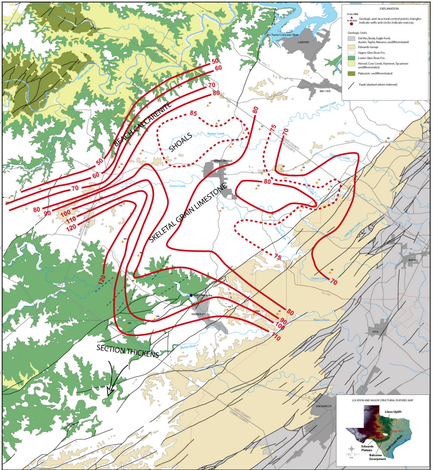
Figure 19. ISOPACH OF THE COW CREEK LIMESTONE March 2007
